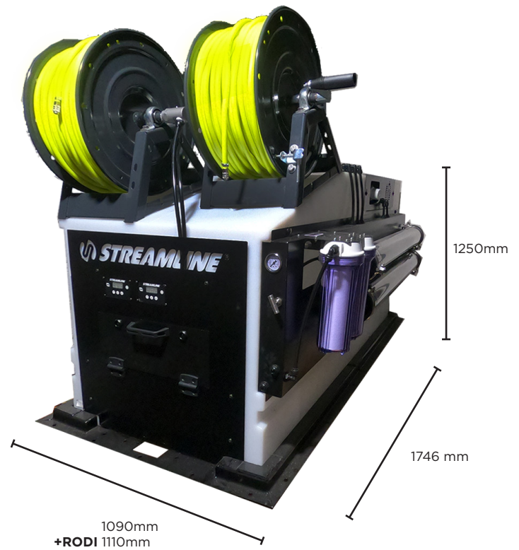
COMBI™700 RODI
